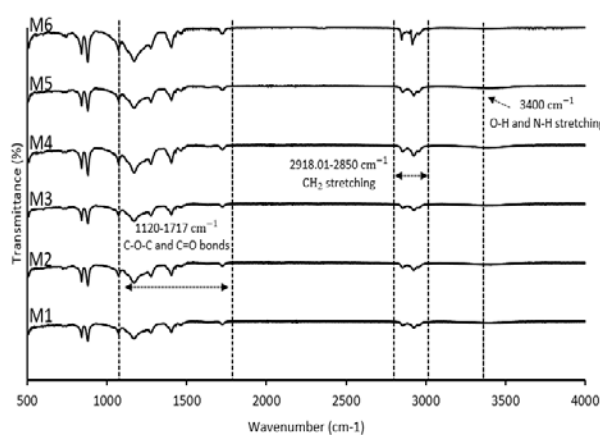
Figure 1 – FTIR spectra of PVDF-co-HFP-based PIMs with different functionalized chitosan (M1-M6)
