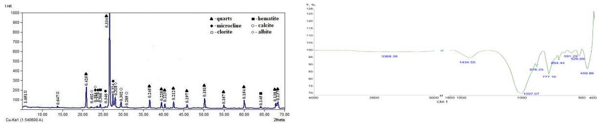
Figure 2 - X-ray Diffraction Pattern and IR Spectrum of the Feldspar-Quartz Sand Sample from the Khiva Deposit
